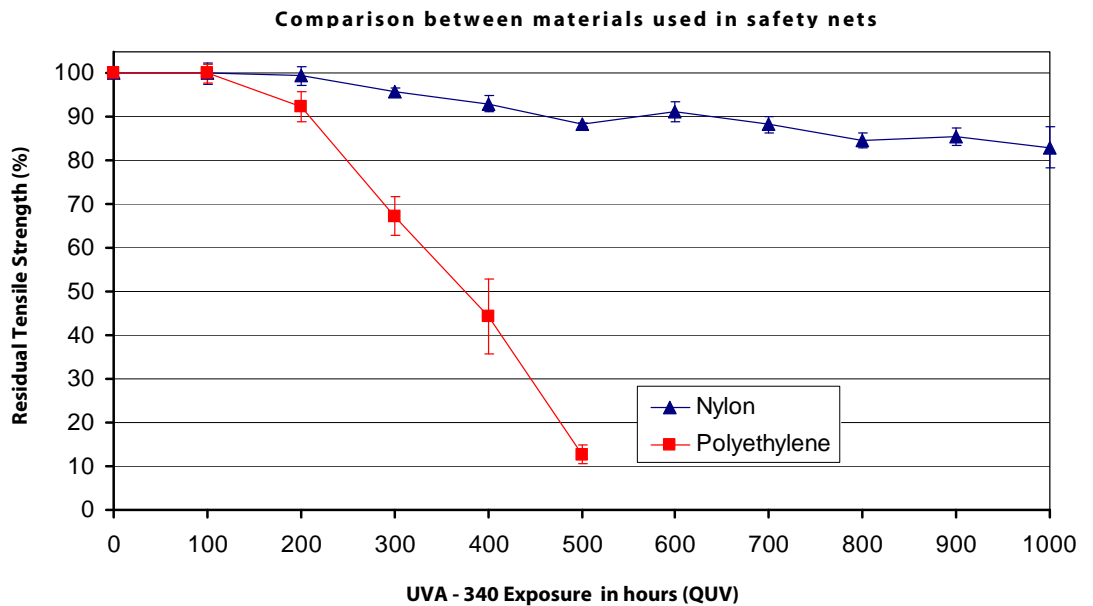
Fig.1. Residual tensile strength after exposure in QUV chamber (Ref. document 020411-2)
