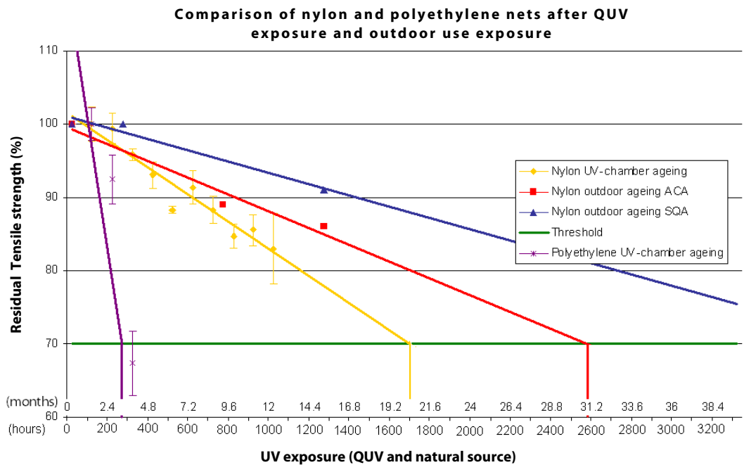
Fig.2. Residual tensile strength after exposure in QUV chamber and after exposure to intensive outdoor use.
